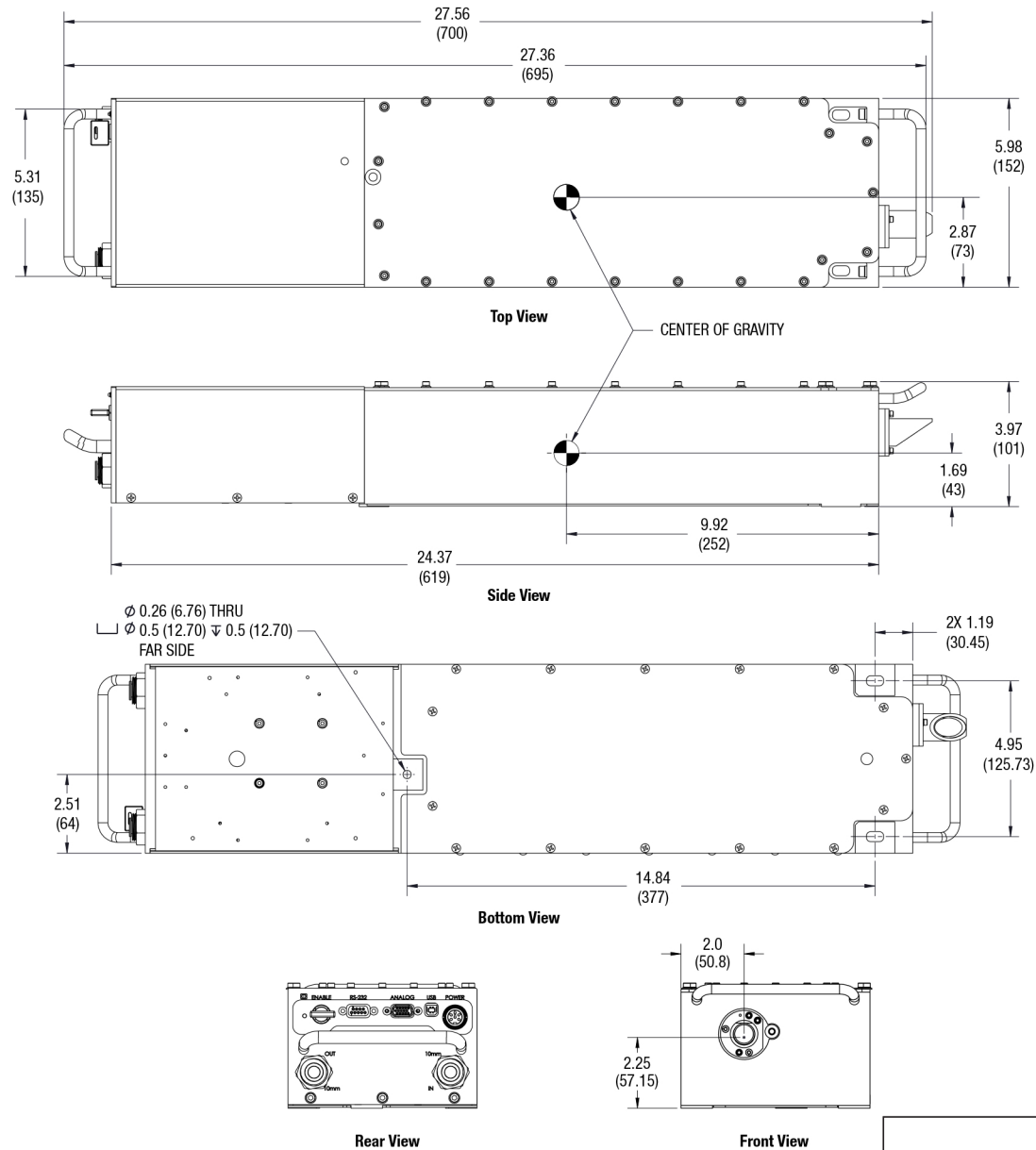
Talon Mark Dimensions
