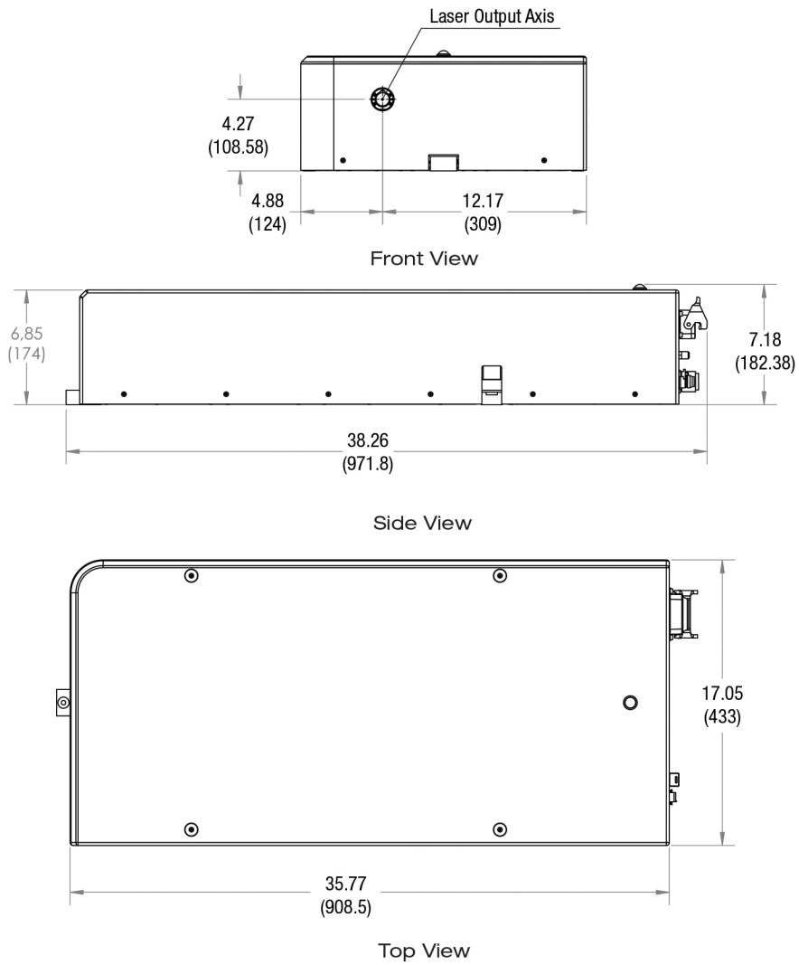
IceFyre FS Laser Dimensions
