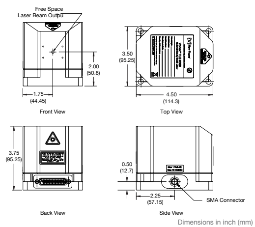
Vortex Plus TLB-6800 Dimensions, Free Space, No Isolator
