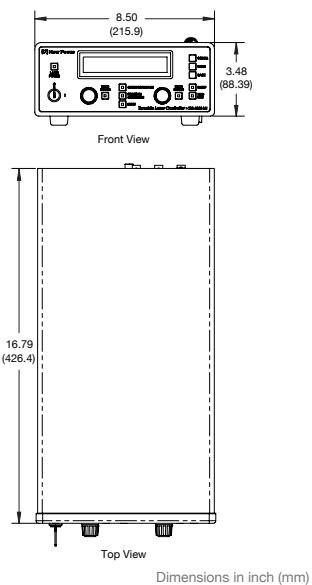
TLB-6800-LN Controller Dimensions
