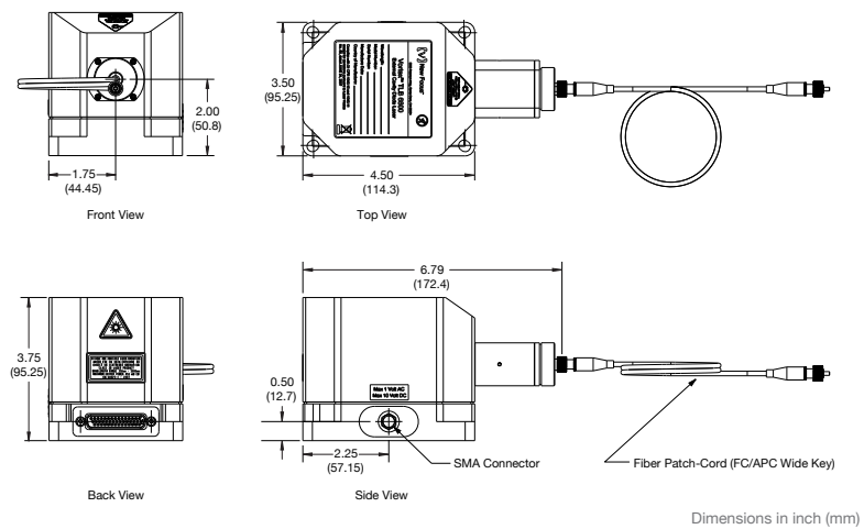
Vortex Plus TLB-6800 with Fiber Dimensions
