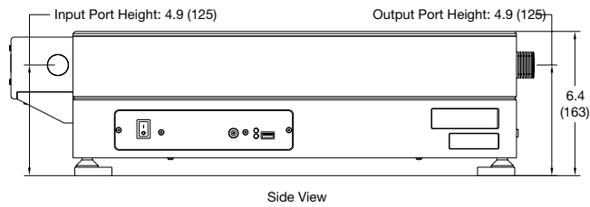
Spirit-OPA-8 Dimensions
