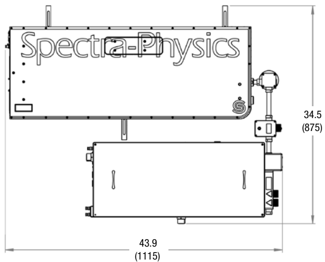
Spirit 1030-70/100 pumping Spirit-NOPA-VISIR Dimensions (without Signal compressor, top view)
