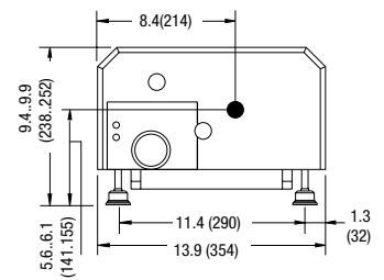
Pump Laser Input End
