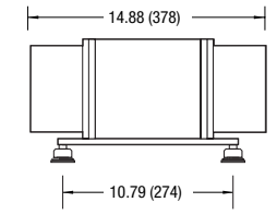
Matisse DS and TS Reference Cell (Side View)
