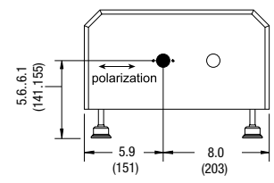
Matisse Output End
