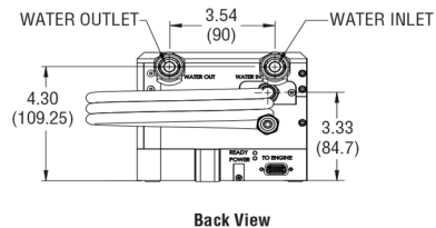
SPFL 532-40 Laser Head Dimensions
