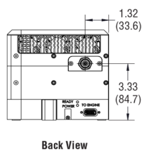
SPFL 532-20 Laser Head Dimensions
