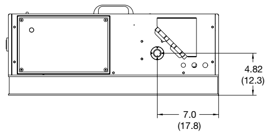
Pump End View
