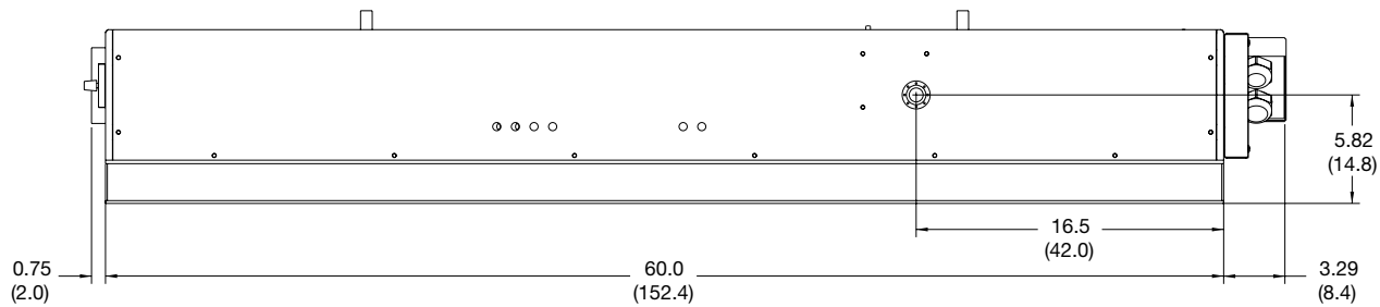
Side View, Seed Input Panel
