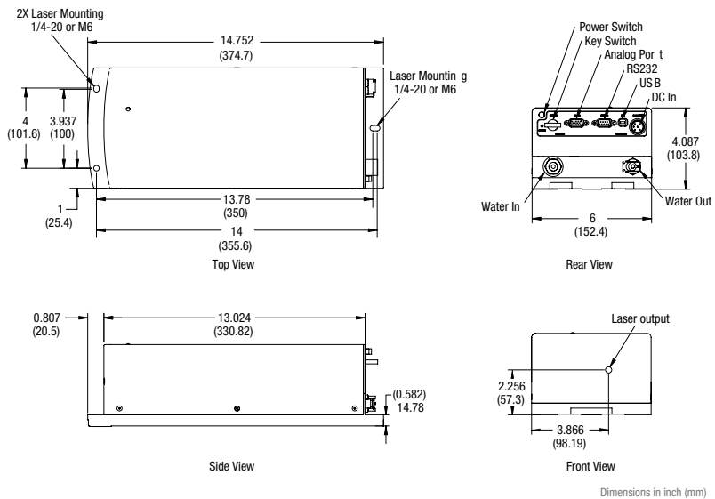
Millennia eV (5-15 W) Dimensions
