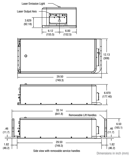
IceFyre IR50 Laser Dimensions
